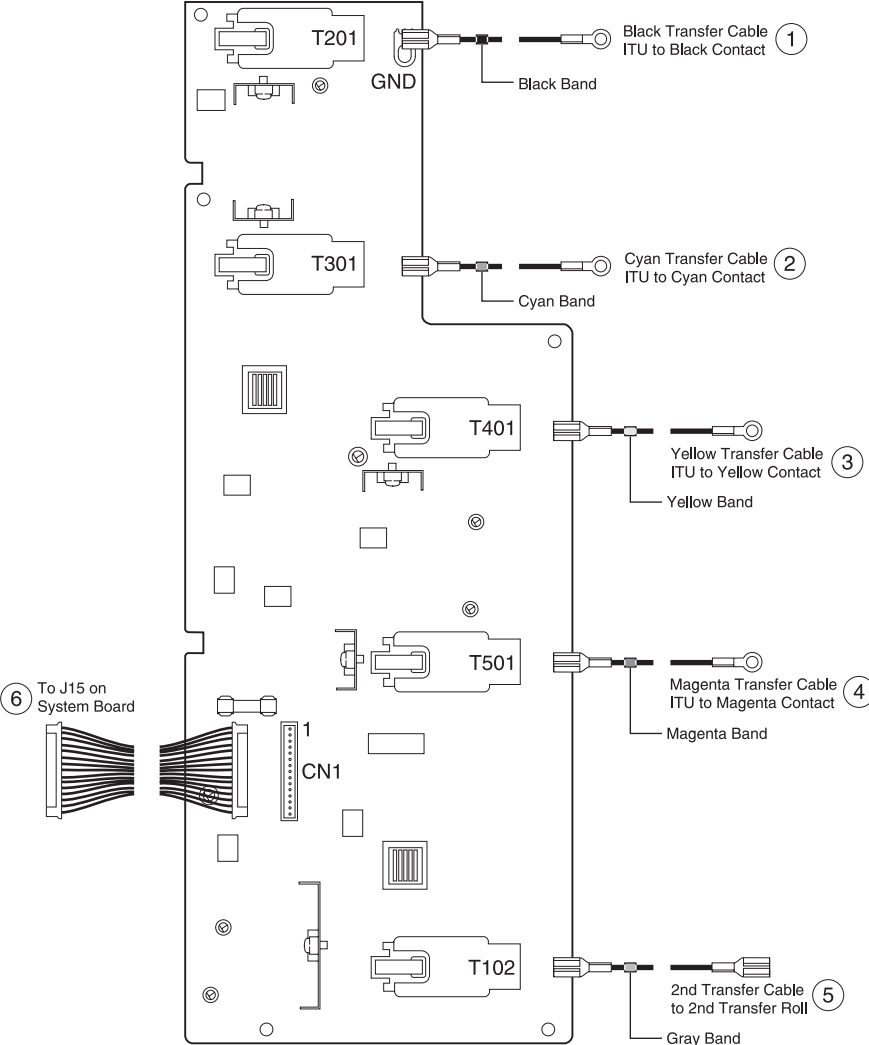
Transfer HVPS
